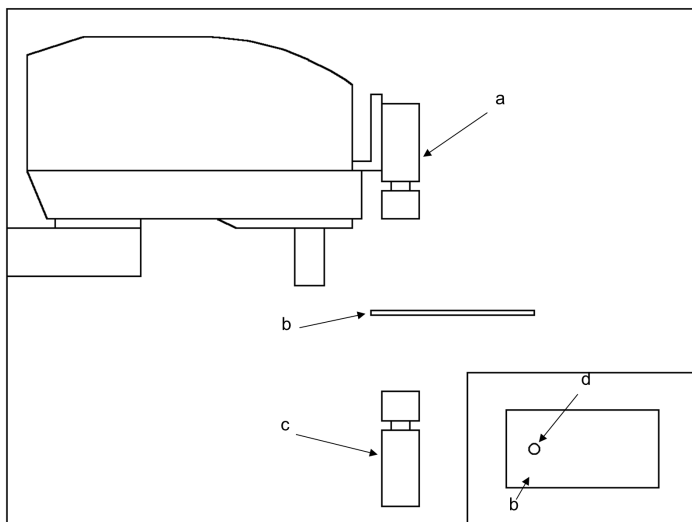
Mobile Camera Calibration using Fixed Upward Camera
