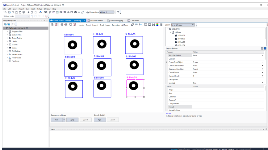
Vision objects placed in order for Standalone Camera Calibration
